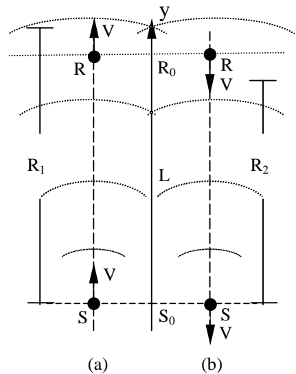
Fig. 3 Moving frames
